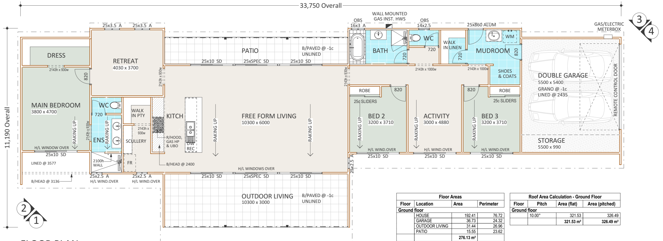
FLOOR PLAN 1:100
