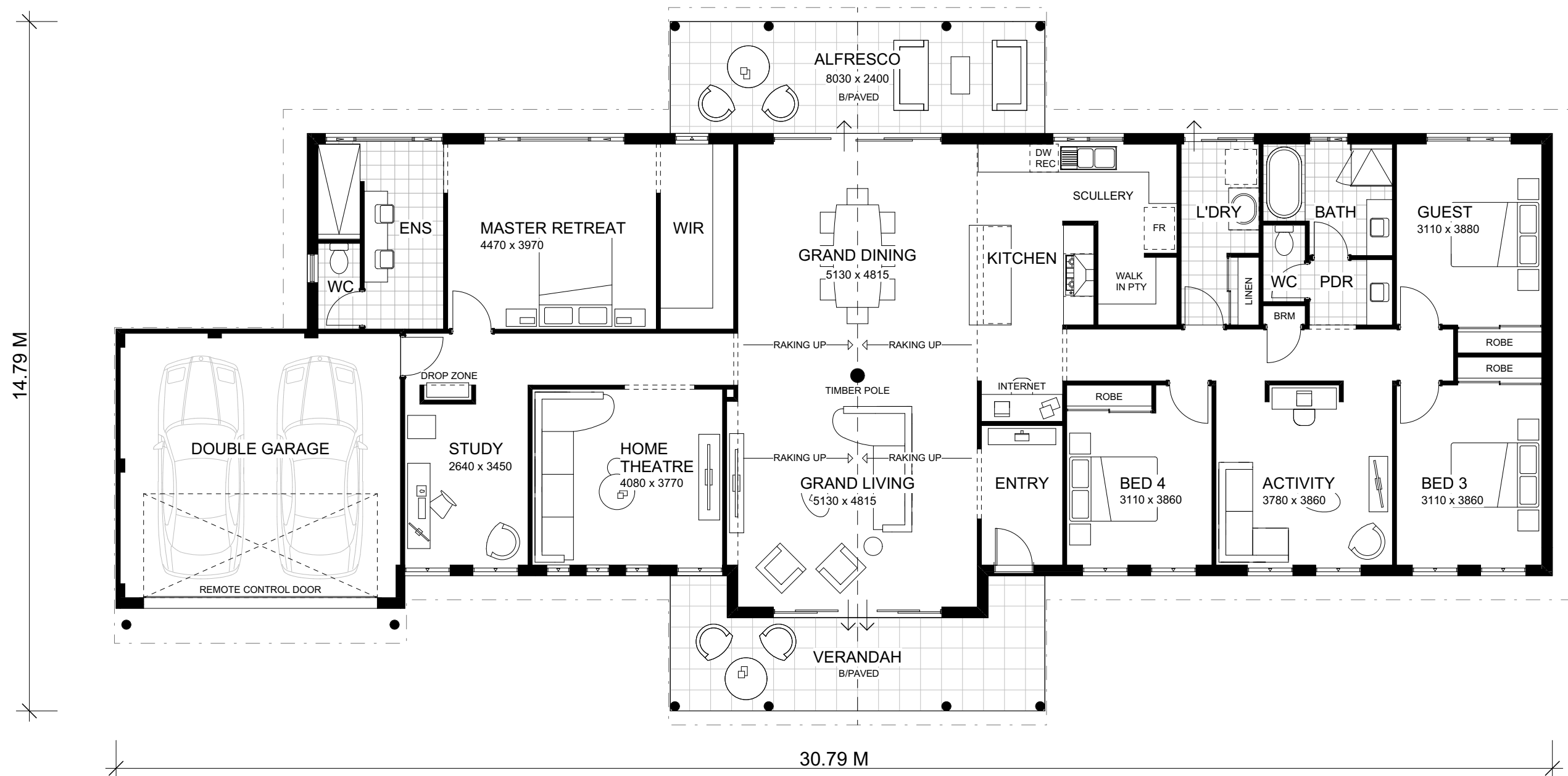
FLOOR PLAN 1:100
