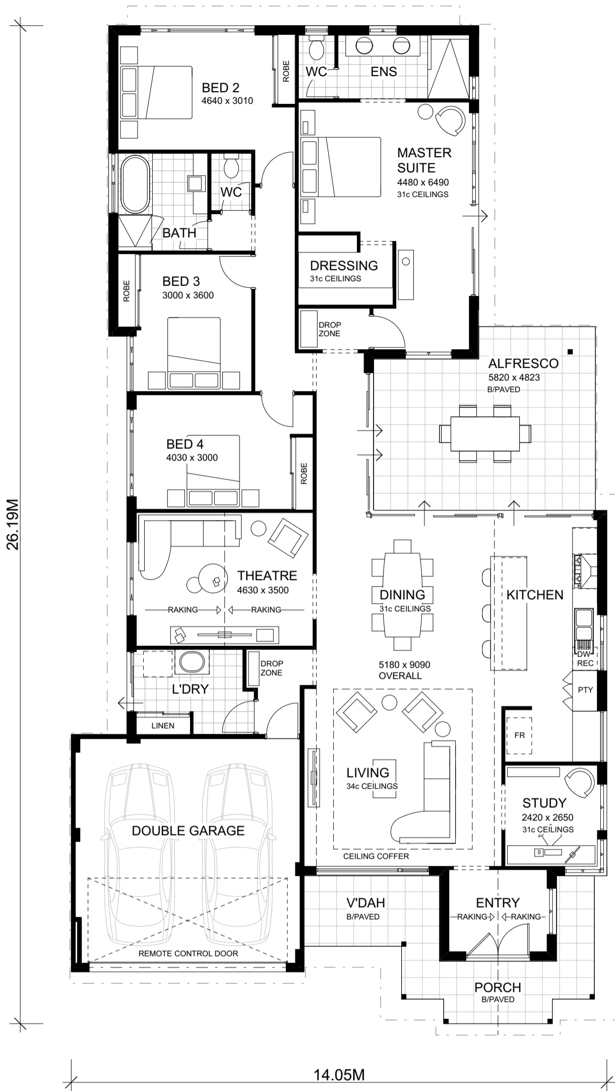
FLOOR PLAN 1:100
