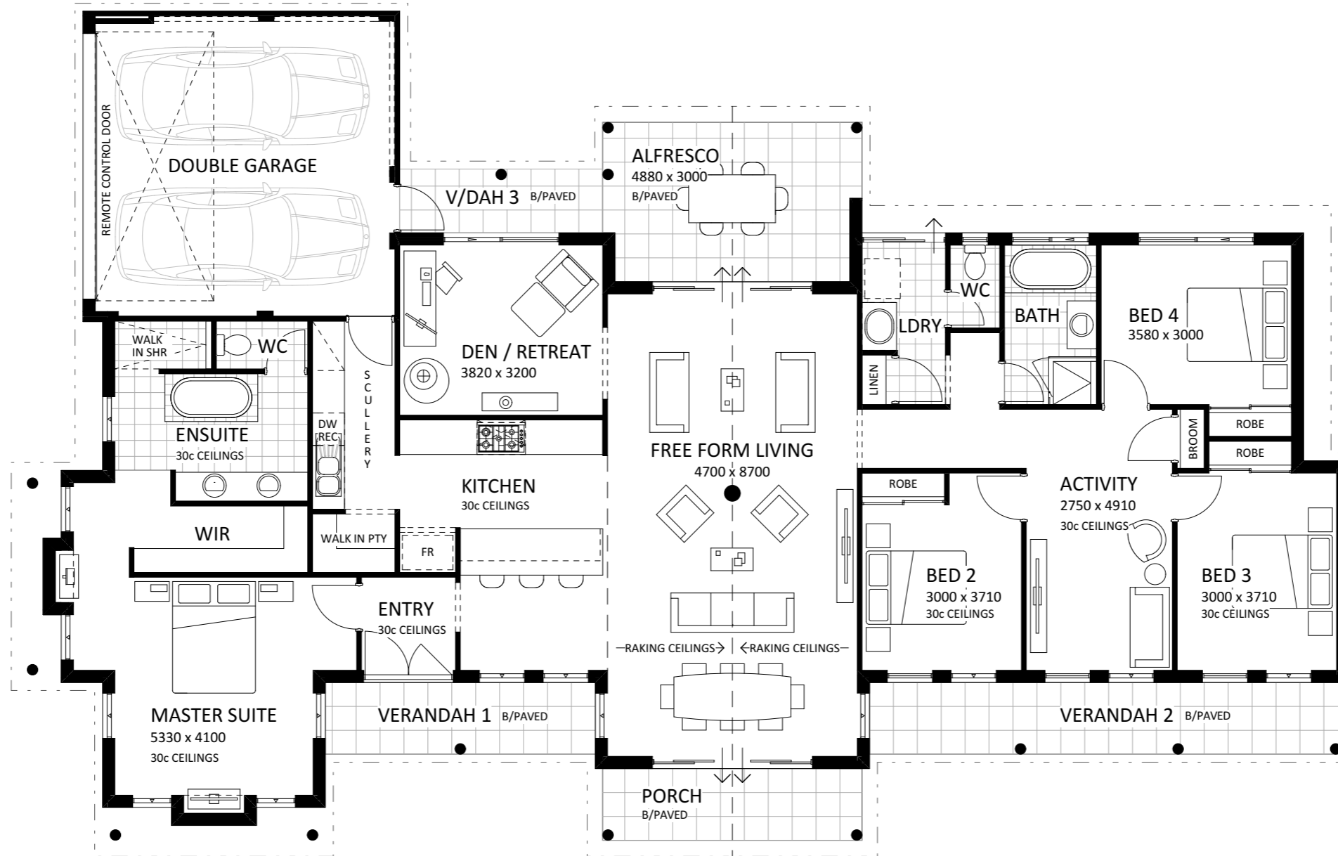
FLOOR PLAN 1:100
