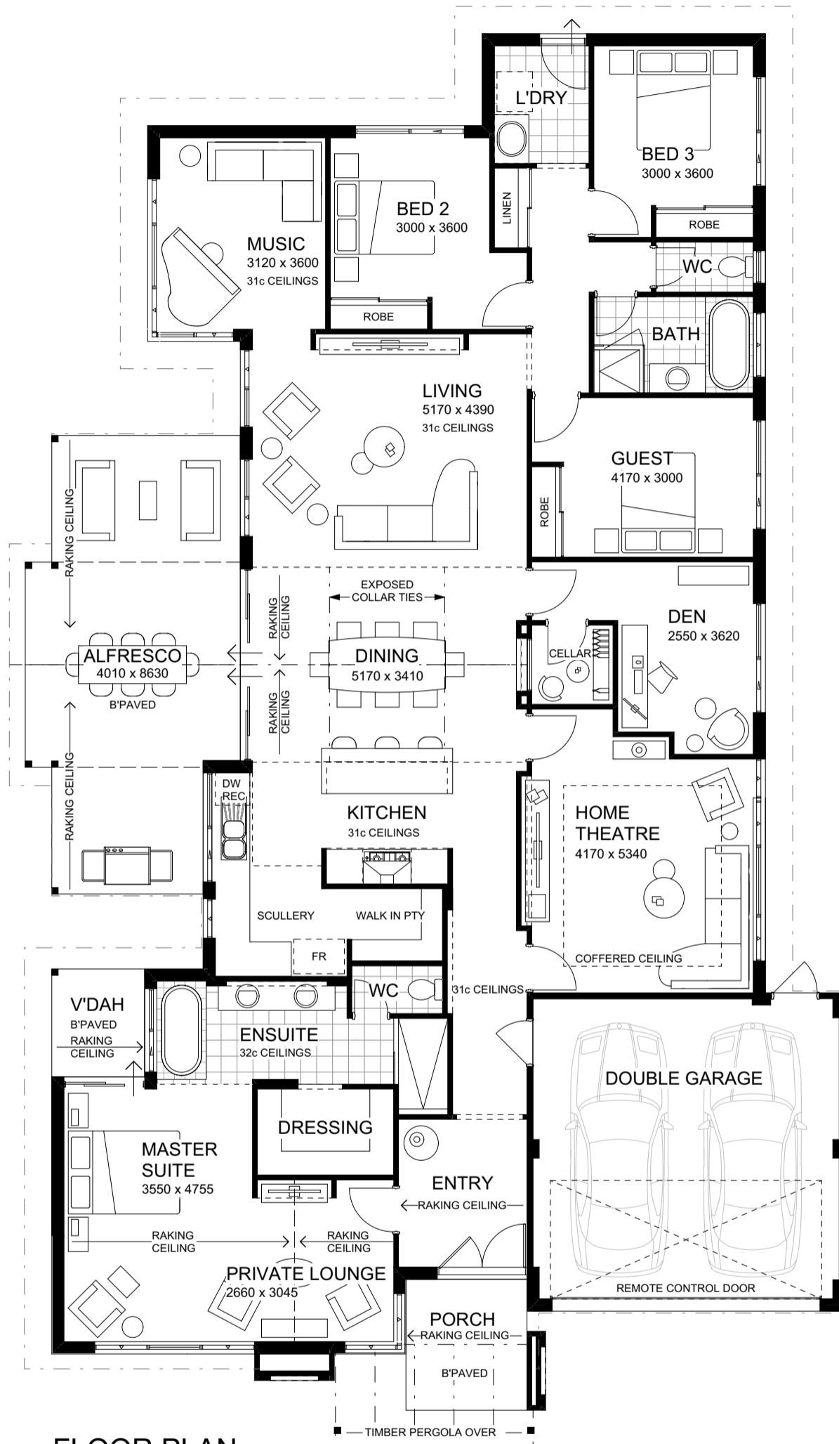
FLOOR PLAN 1:100
