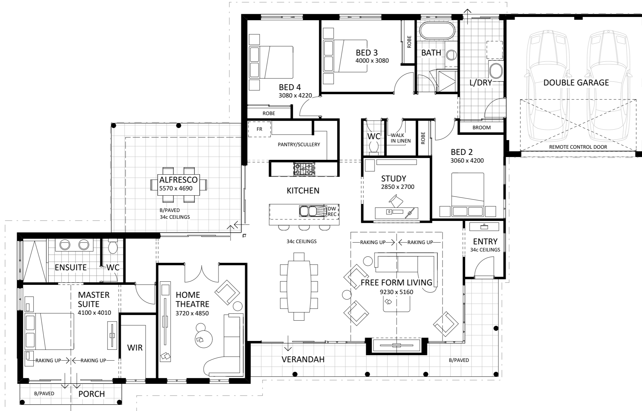
FLOOR PLAN 1:100
