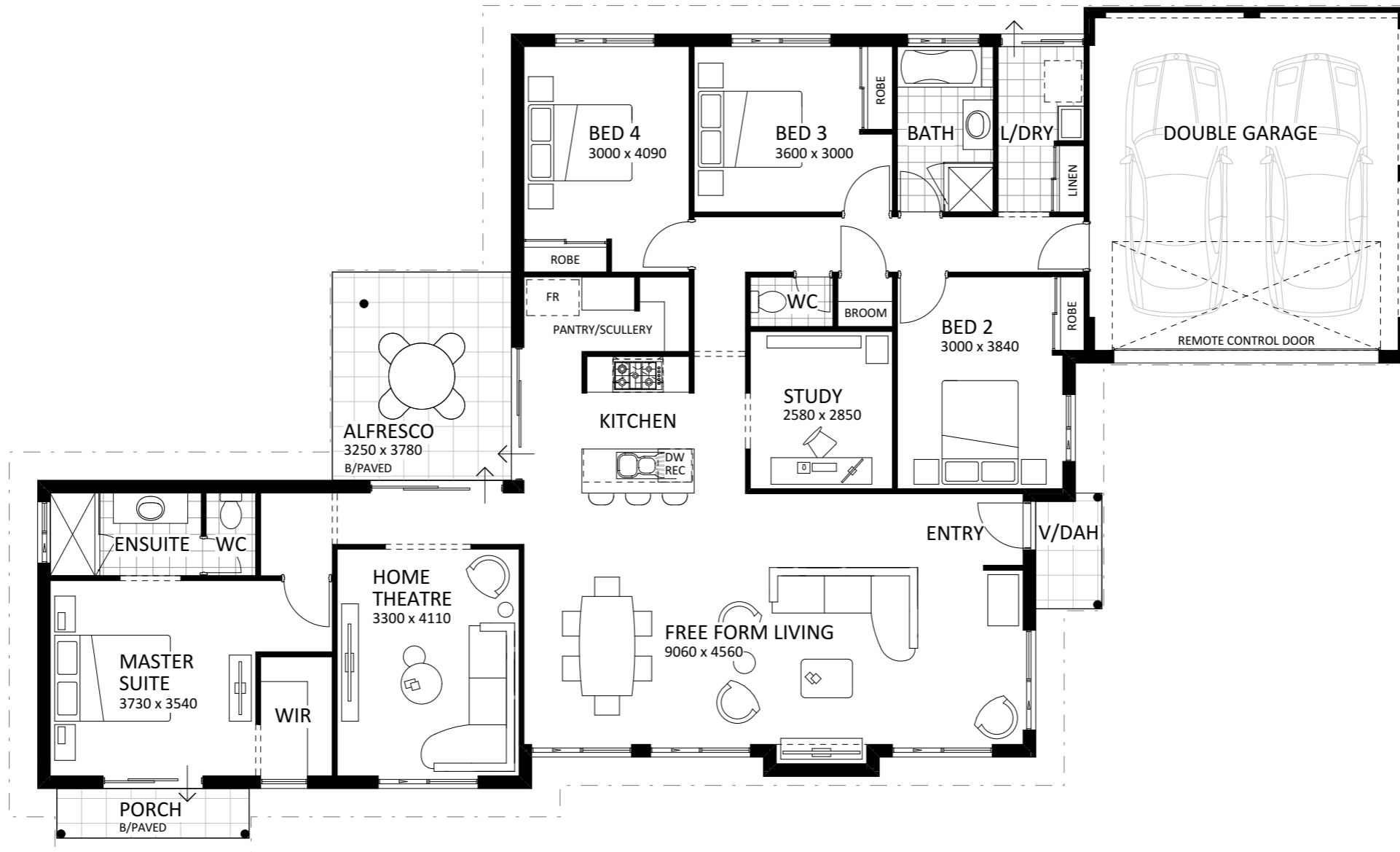
FLOOR PLAN 1:100
