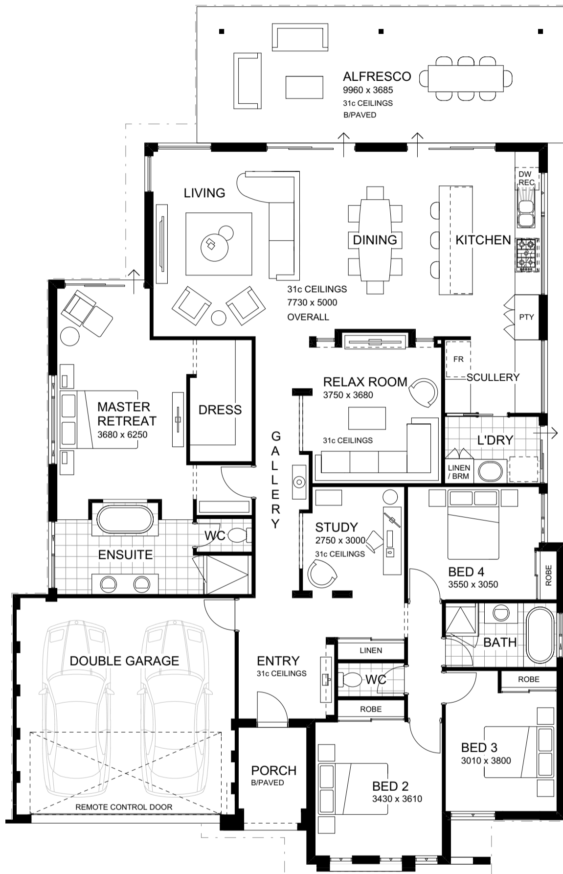
FLOOR PLAN 1:100
