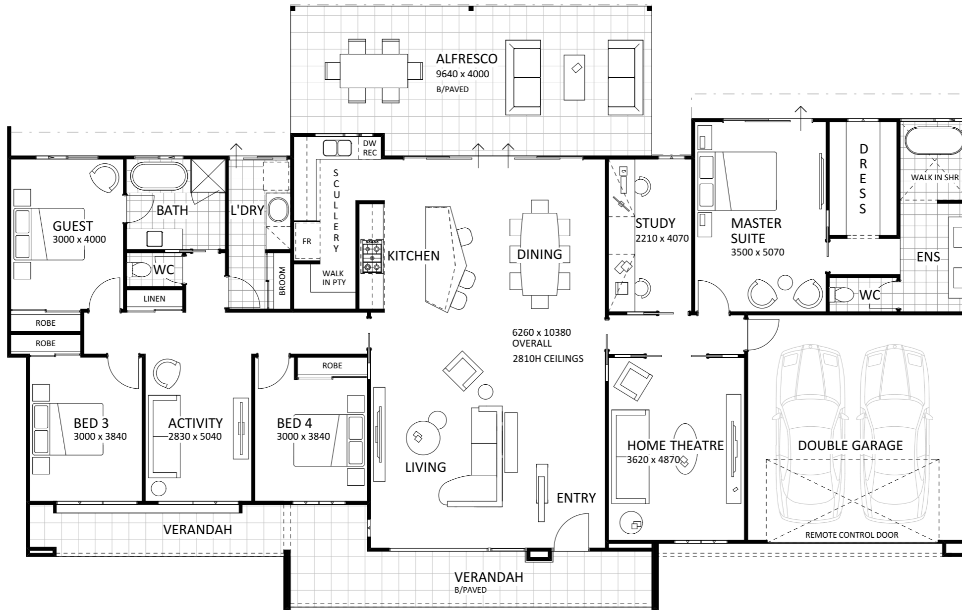
FLOOR PLAN 1:100
