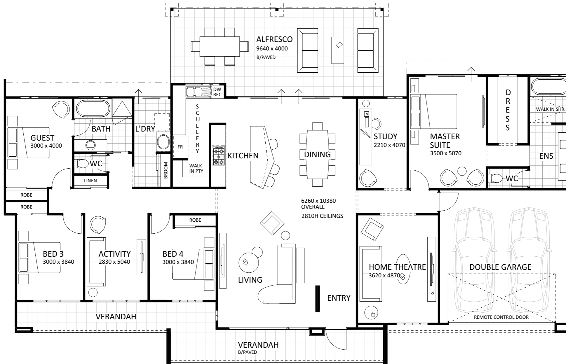
FLOOR PLAN 1:100
