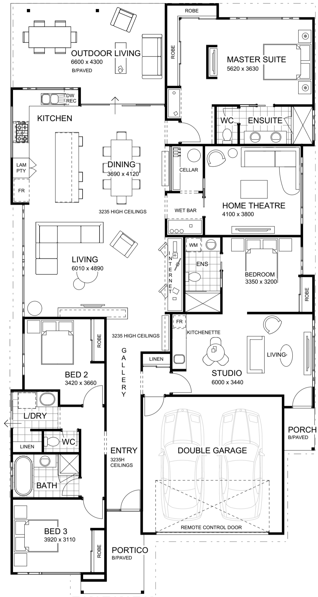
FLOOR PLAN 1:100
