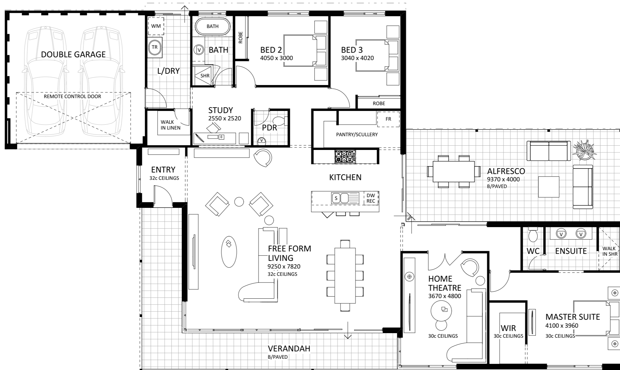
FLOOR PLAN 1:100
