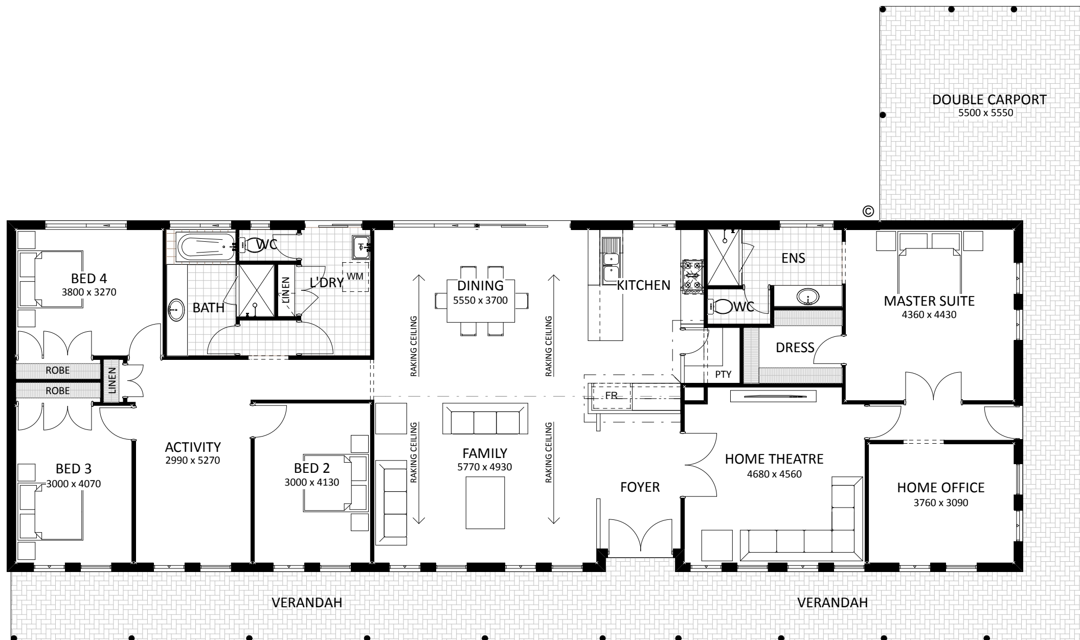
FLOOR PLAN 1:100
