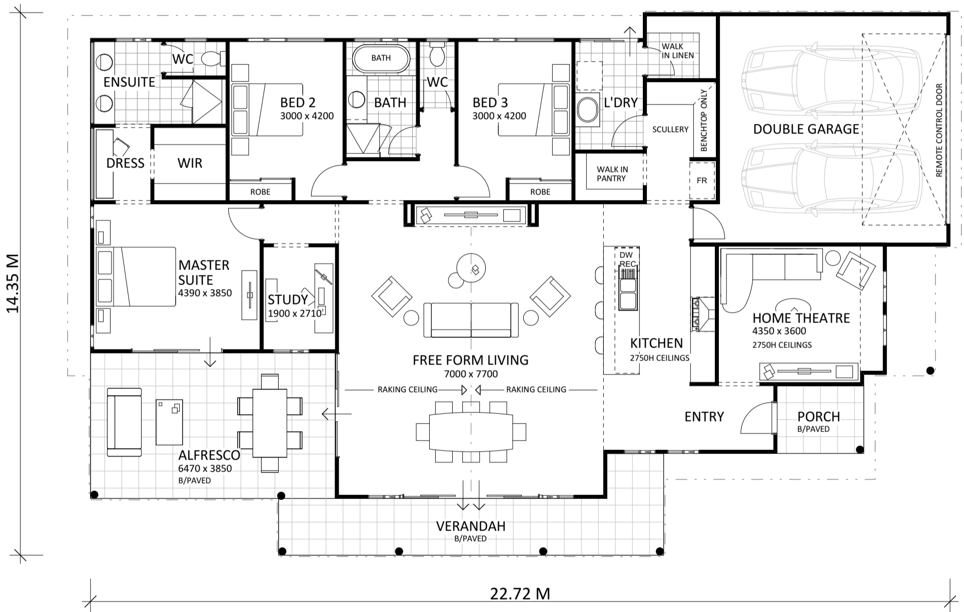
FLOOR PLAN 1:100
