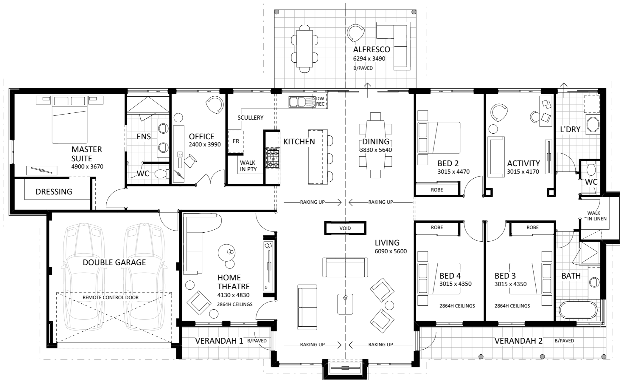
FLOOR PLAN 1:100
