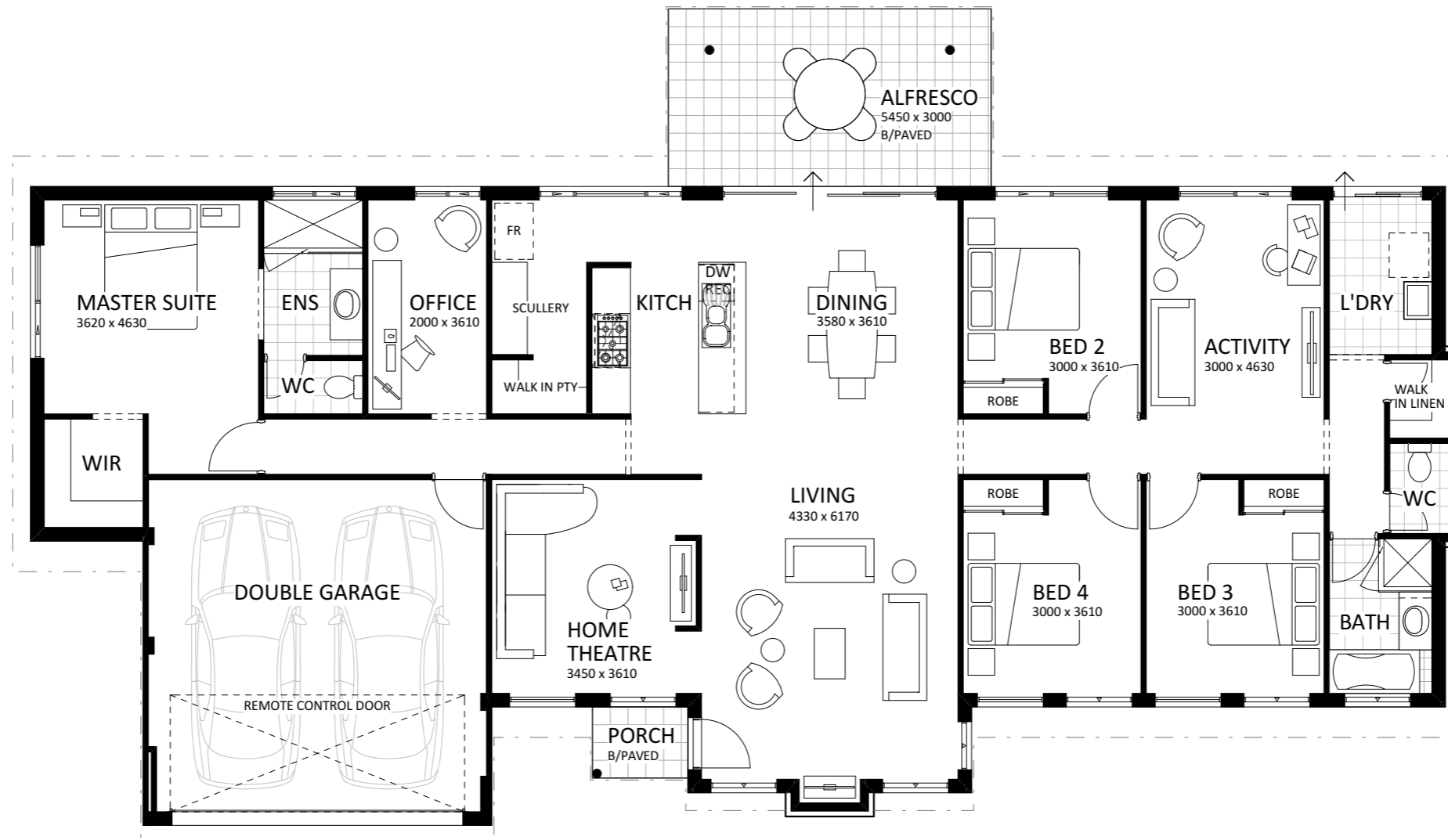
FLOOR PLAN 1:100
