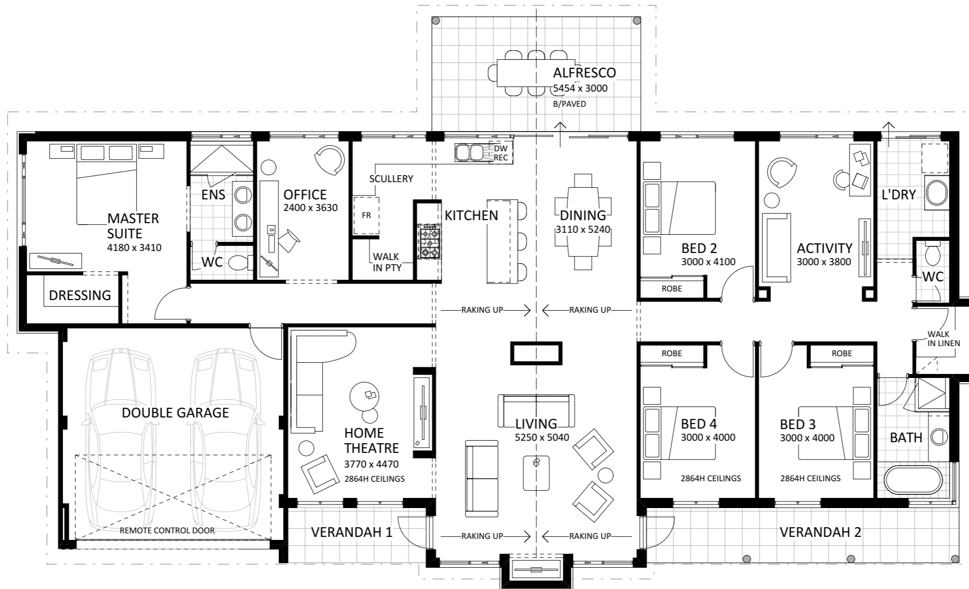
FLOOR PLAN 1:100
