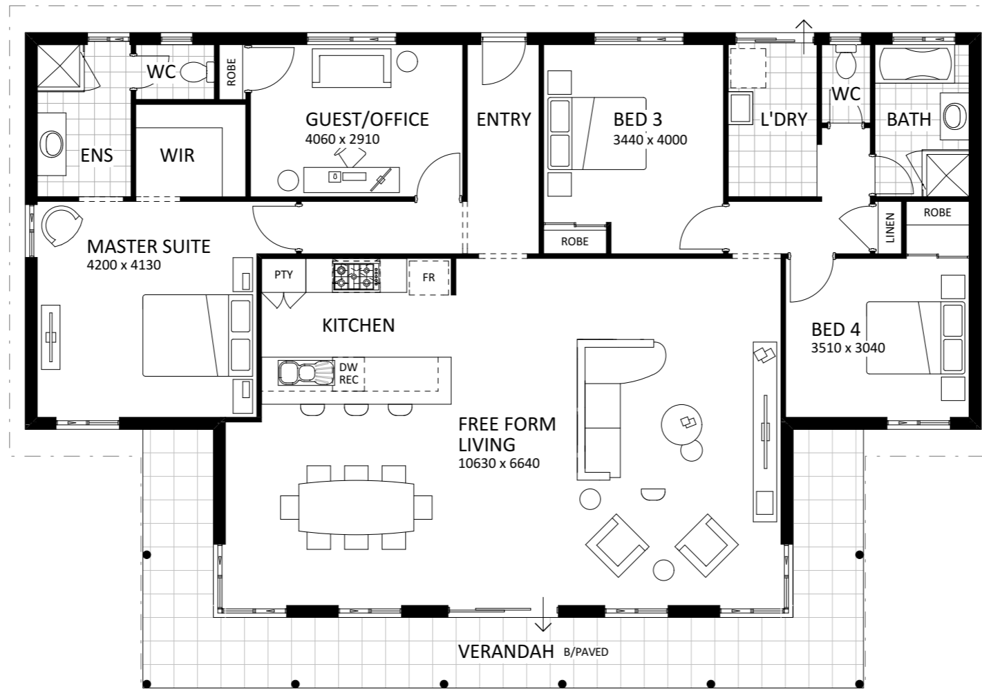
FLOOR PLAN 1:100
