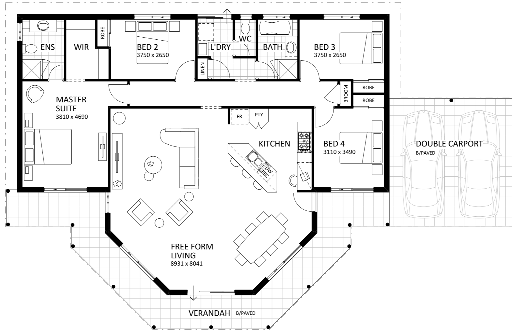
FLOOR PLAN 1:100
