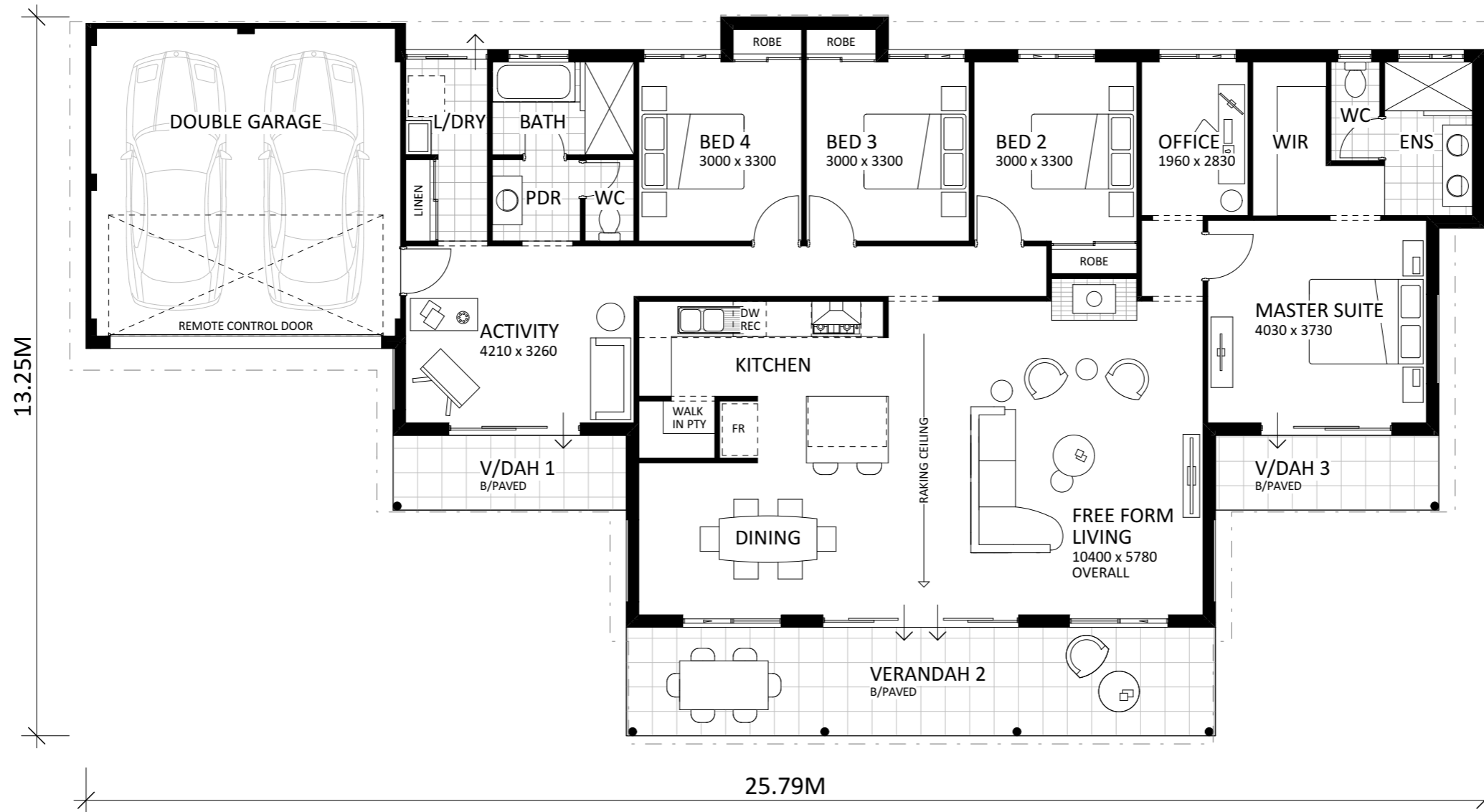
FLOOR PLAN 1:100
