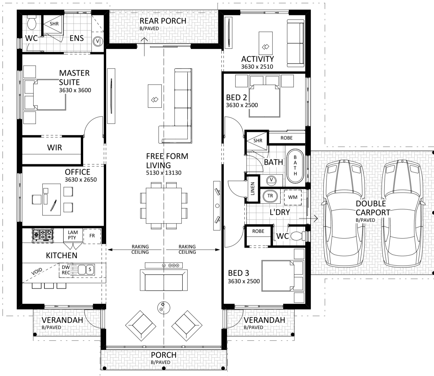
FLOOR PLAN 1:100
