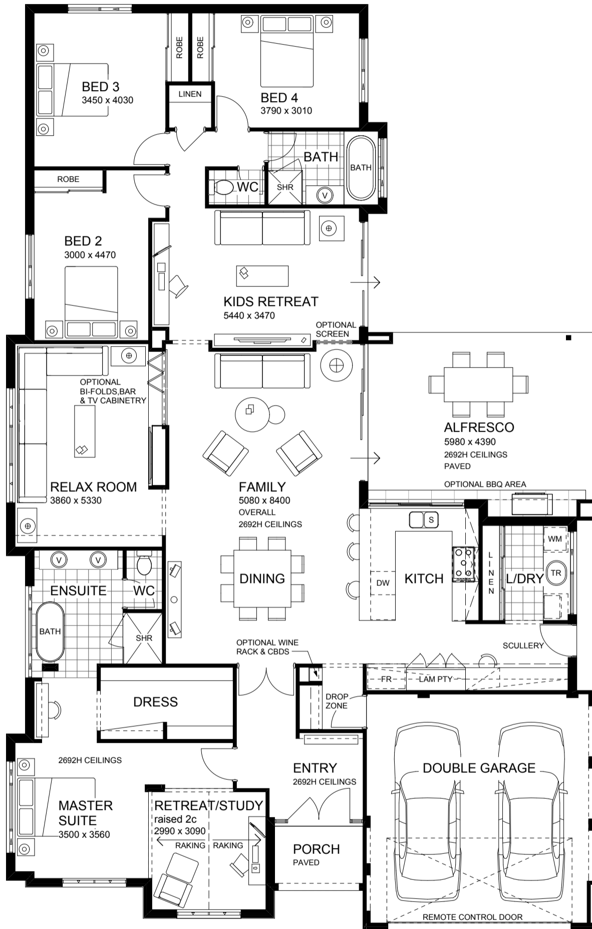
FLOOR PLAN 1:100
