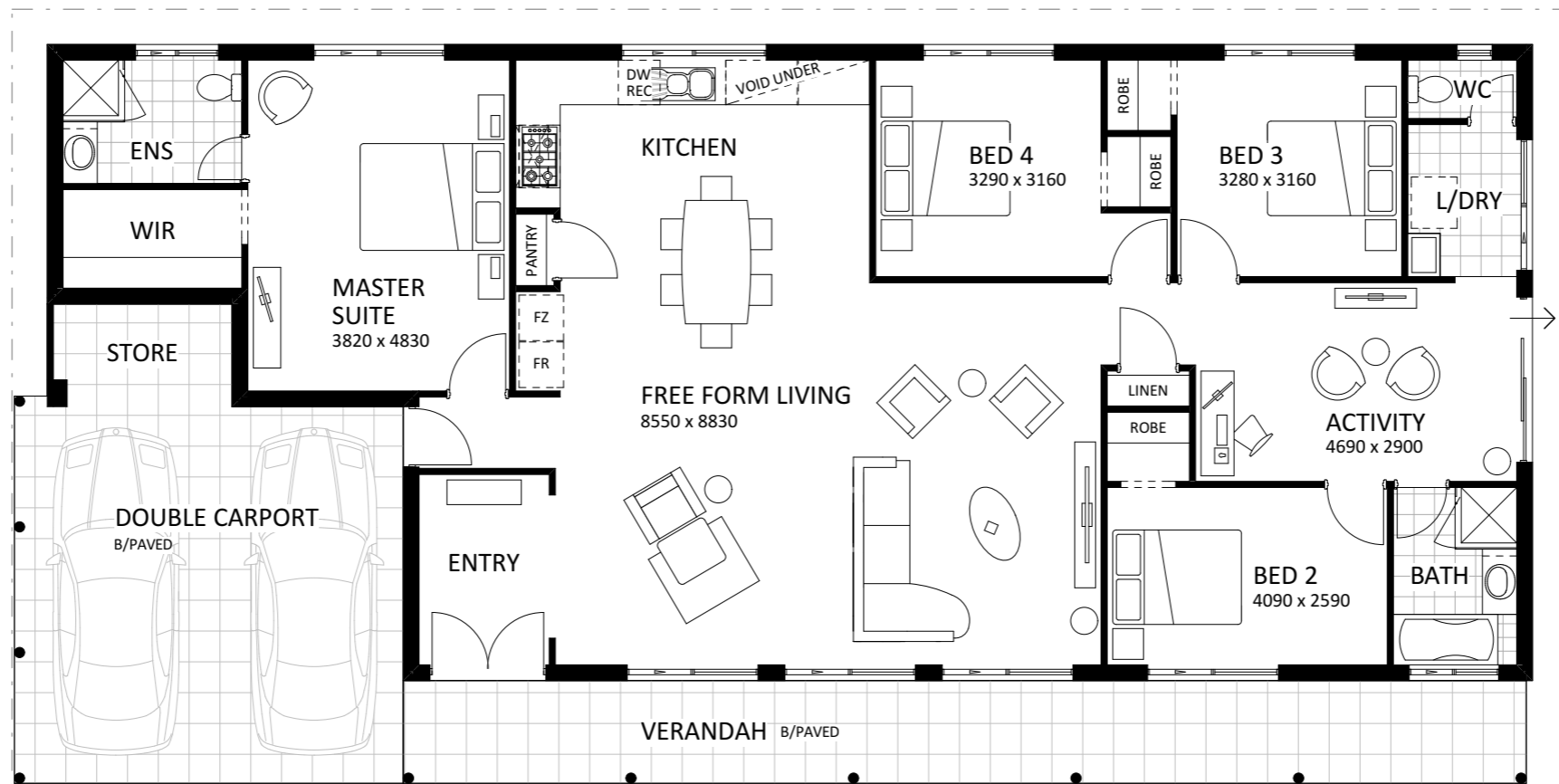
FLOOR PLAN 1:100
