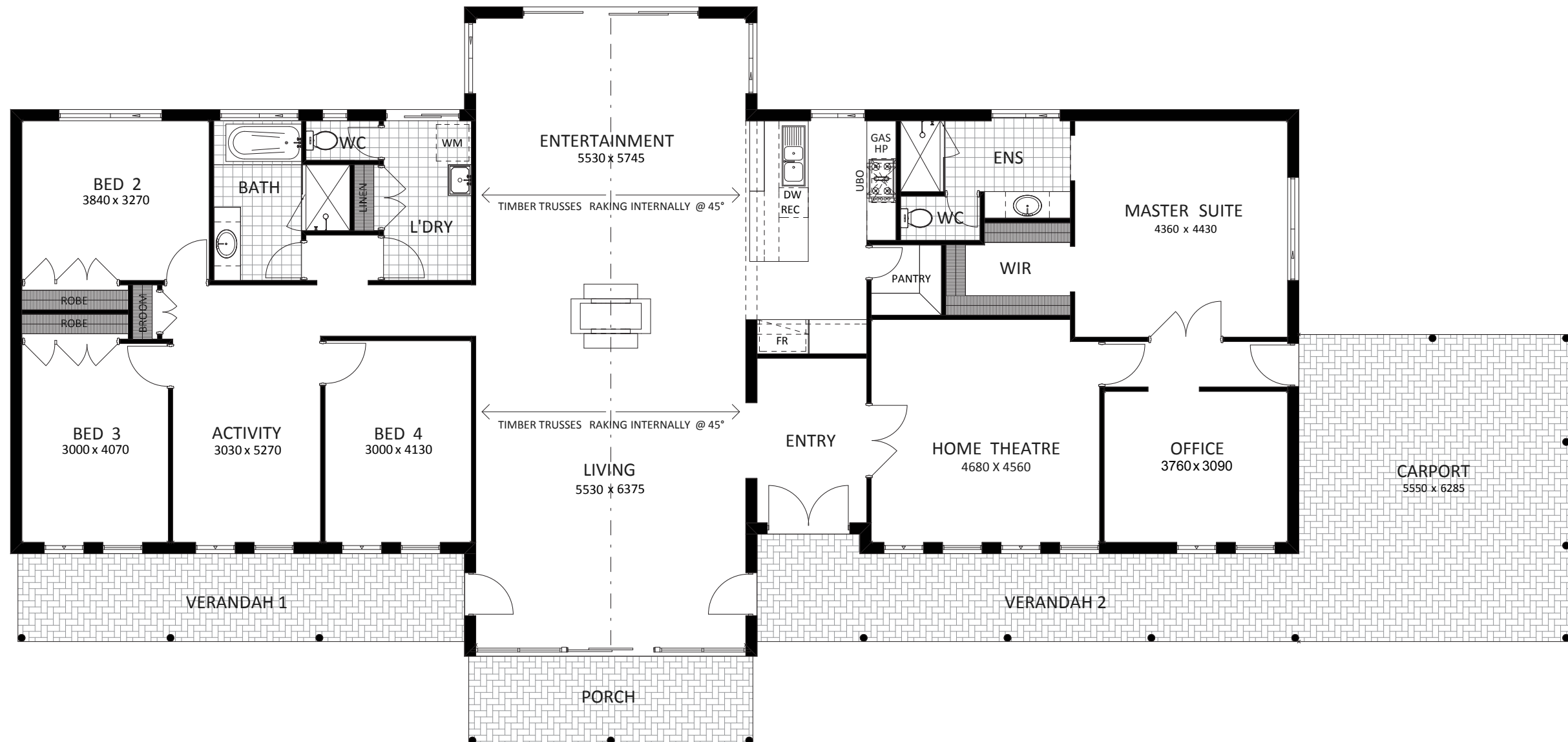
FLOOR PLAN 1:100
