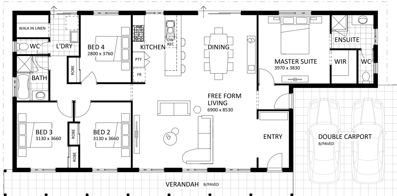
FLOOR PLAN 1:100
