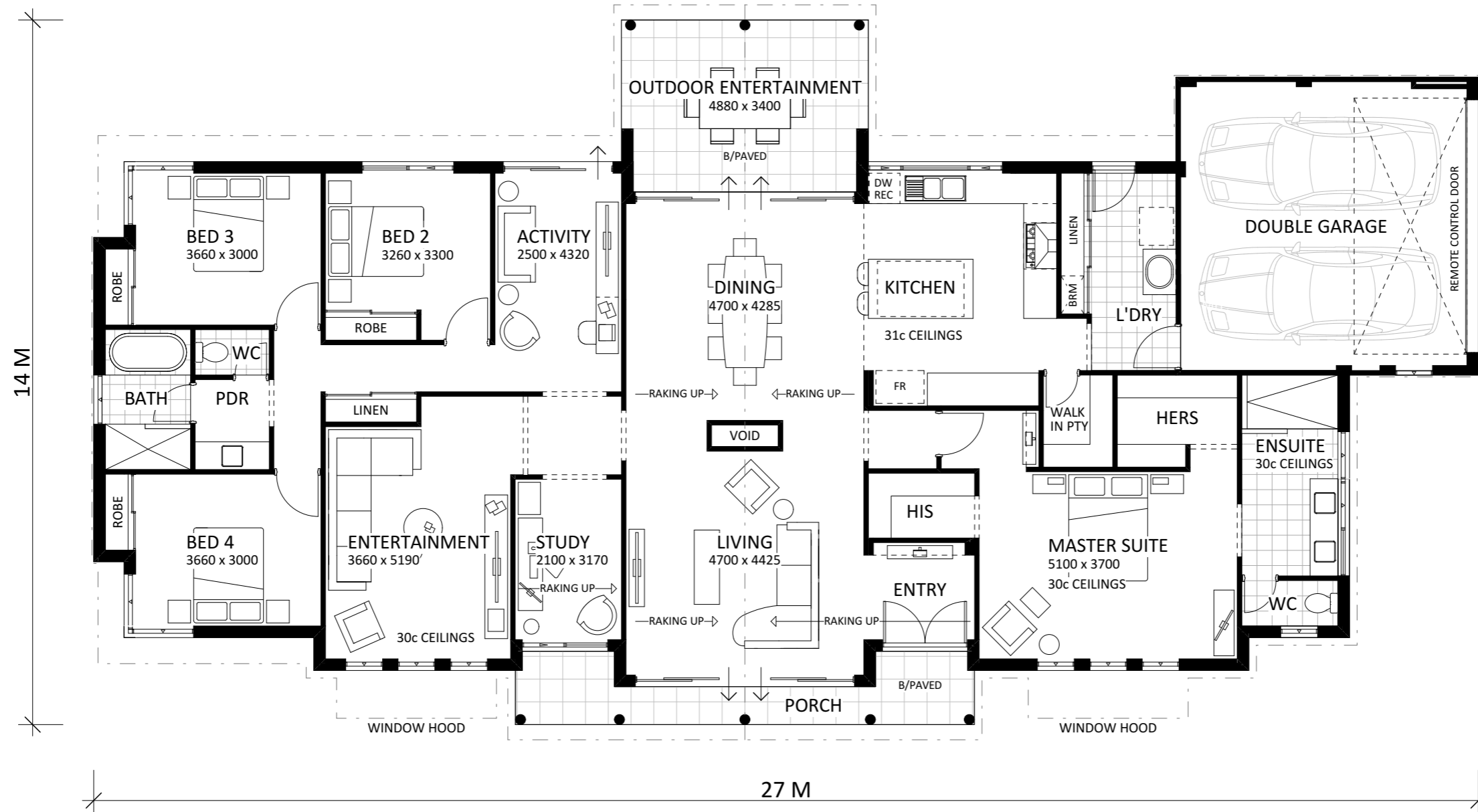
FLOOR PLAN 1:100
