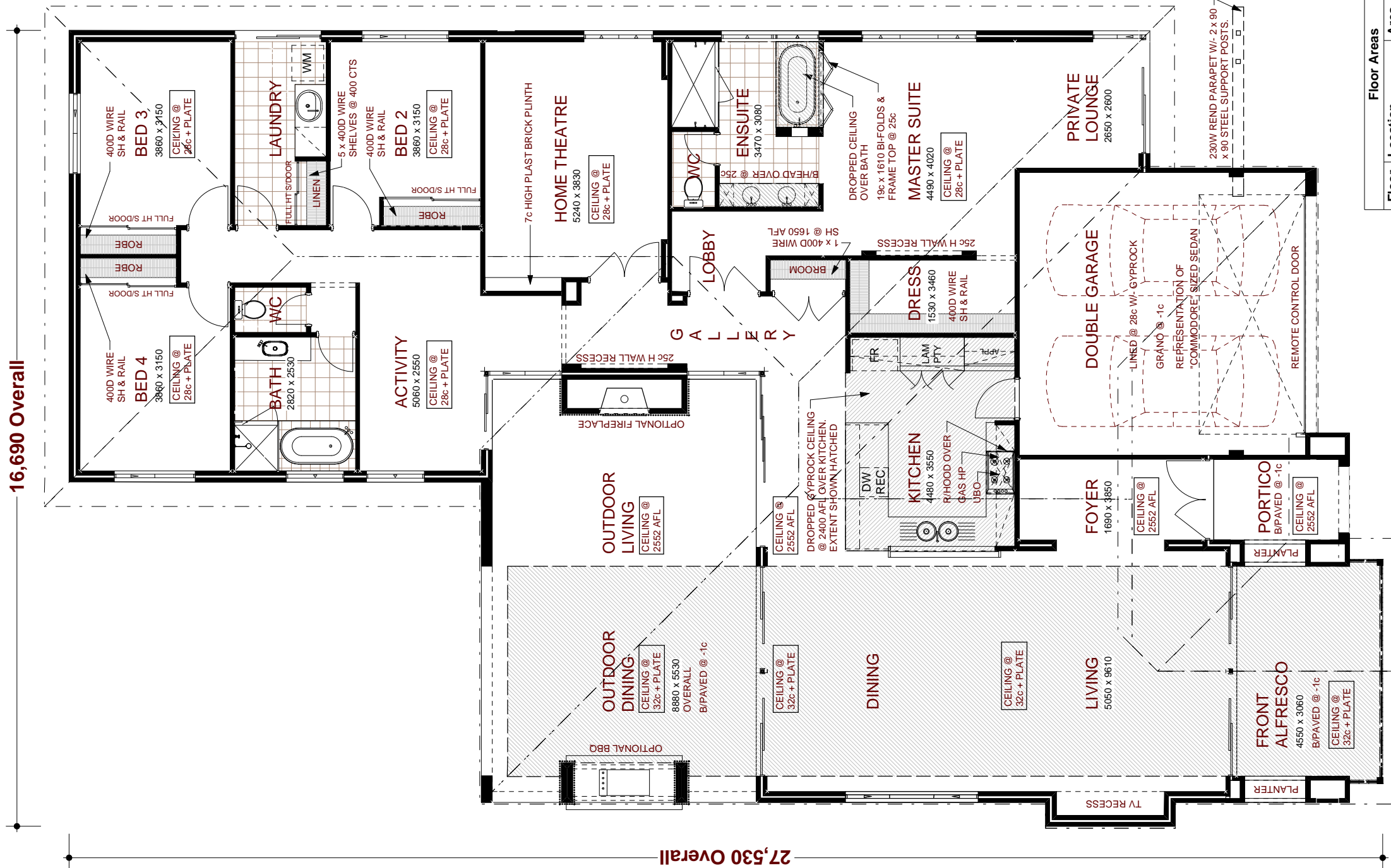
FLOOR PLAN 1:100
